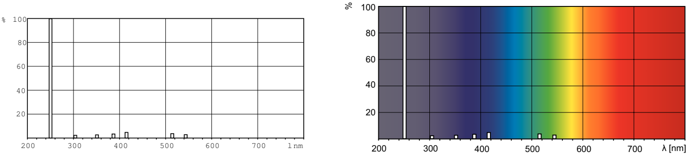
XDPO_XUTUVPLL-Spectral power distribution Colour
